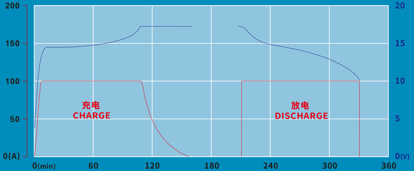
▲ TSWB-LP12V100AH 25 100A TSWB-LP12V100AH CHARGE AND DISCHARGE BY 100A AT TEMPERATURE OF 25
